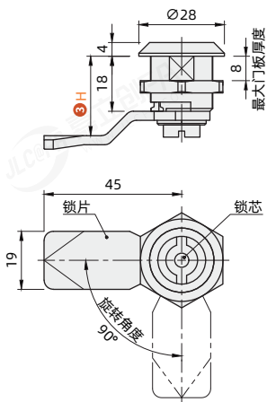
圆形 DMSY-W-5 DMSY-G3-5
